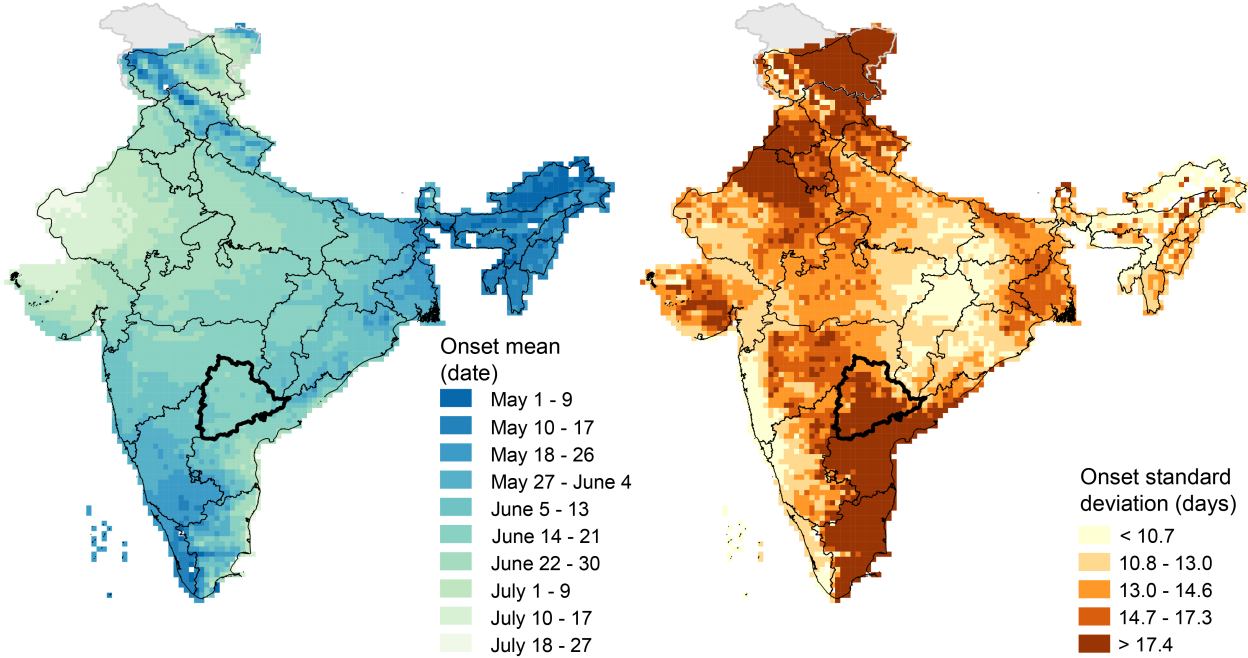
Figure 1: Monsoon onset over India
